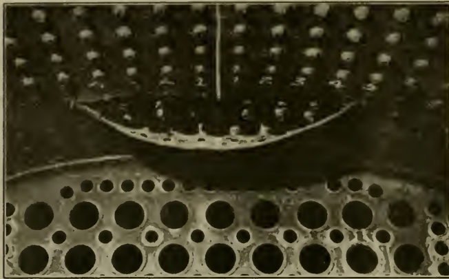
FIG. 7. SHOWING RESULT OF AN EXPLOSION DUE TO LOW WATER.
